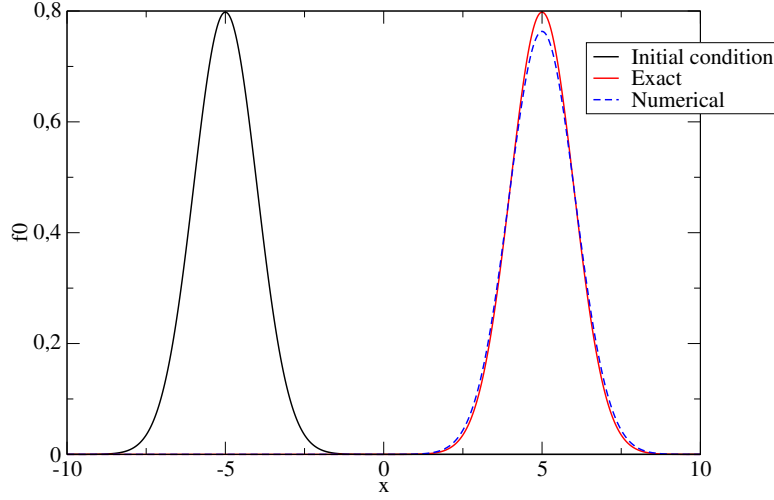
FIGURE 2. Free transport: comparison of the numerical solution for \Delta x = 4 \cdot 10^{-3} and the exact solution (red) at time t=6 .
