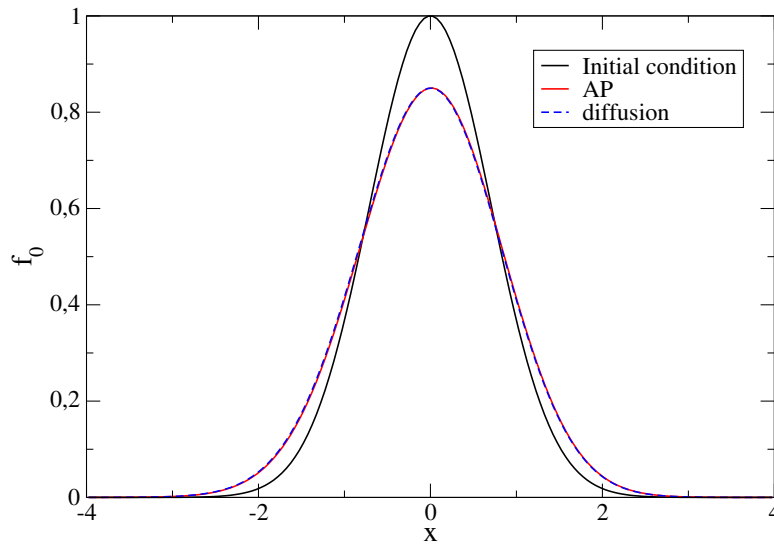
FIGURE 9. Relaxation of a Gaussian profile in the case of a linear collisional parameter: comparison of the f_0 profile for the asymptotic-preserving scheme (AP) and the diffusion solution at time t=150 .
